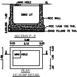
UG SUMP DETAIL
