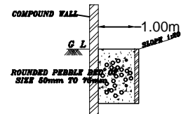
PEBBLE BED DETAILS
