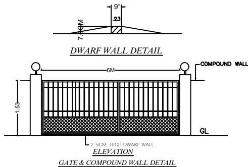
GATE & COMPOUND WALL DETAIL
