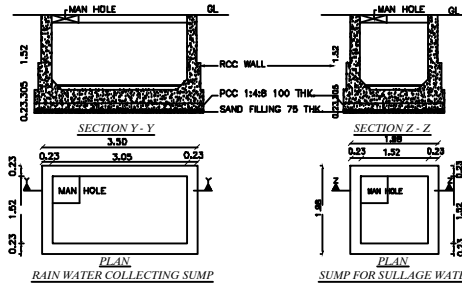
RAIN WATER COLLECTING SUMP
