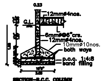
SECTION - R.C.C. COLUMN
